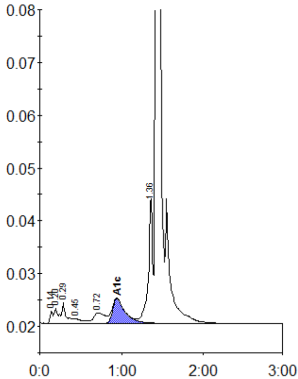
Peak table - ID: 10550823
